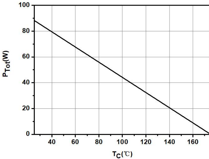
Fig.7-Power Derating
