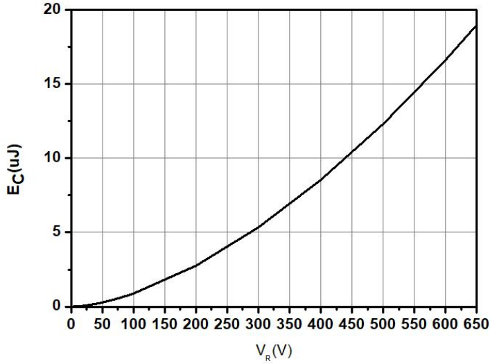
Fig.5-Capacitance Stored Energy
